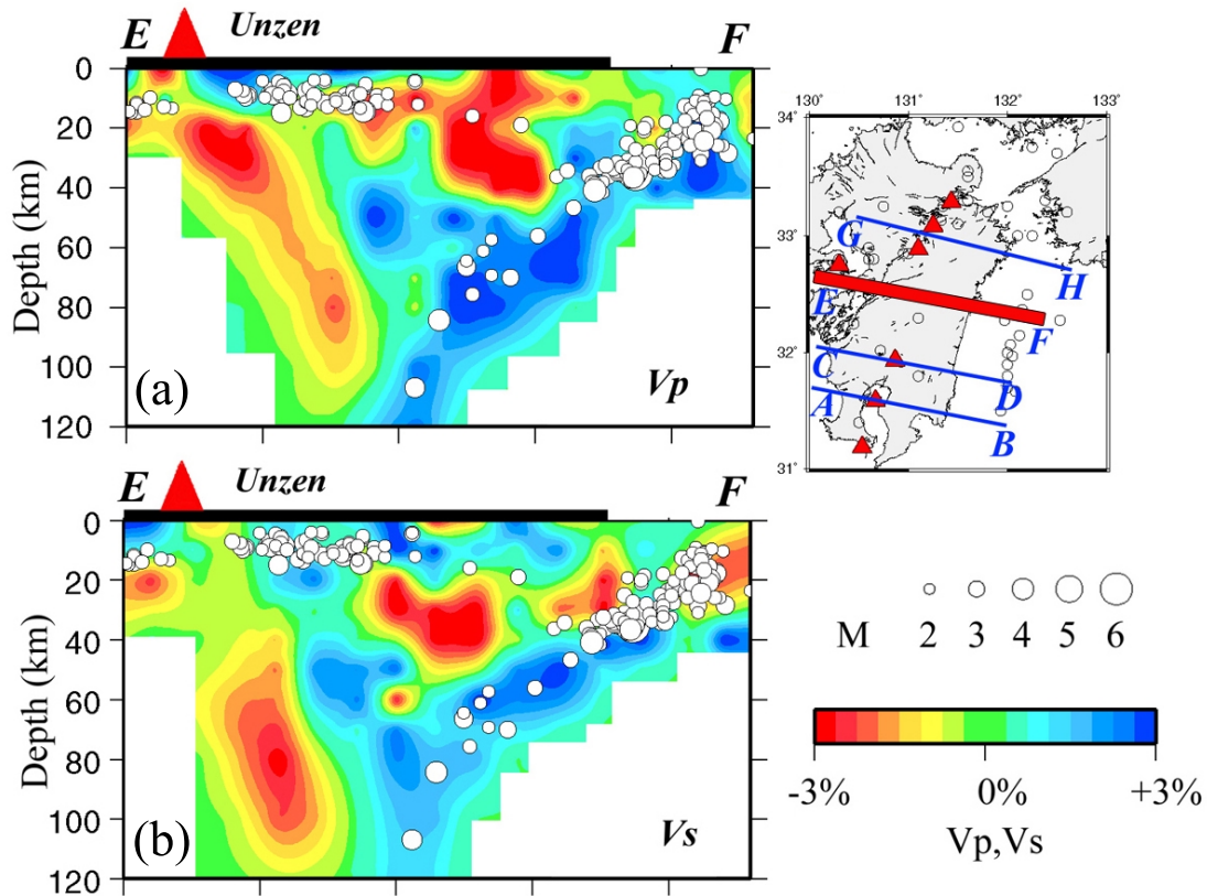
Fig. 19. The same as Fig. 14(a, b) but along profile E-F as shown on the inset map of Kyushu Island. (Reprinted from Phys. Earth Planet. Inter. , 157, Wang, Z., and D. Zhao, V_p and V_s tomography of Kyushu, Japan: New insight into arc magmatism and forearc seismotectonics, 269–285, Copyright 2006, with permission from Elsevier.)
