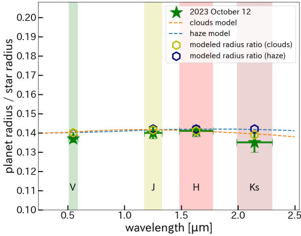
Fig. 5. Observed planet-to-star radius ratios of Qatar-1 b on October 12 compared to cloud and haze model spectra. The green stars represent the radius ratios observed on 2023 October 12. The orange dashed line represents a cloud model spectrum with \text{H}_2 99%, \text{NH}_3 1%, a mean molecular weight of 2.15 g/mol, planetary diameter of 114,100 km (0.7 times the original), an expansion factor b_s of 10, the cloud particle diameter of 1.0 \mu\text{m} , the mass abundance of clouds relative to the entire atmosphere of 1%, and the pressure of 1.0 \times 10^{-5} bar. The blue dashed line represents a haze model spectrum with \text{H}_2 99%, \text{NH}_3 1%, a mean molecular weight of 2.15 g/mol, planetary diameter of 130,400 km (0.8 times the original), an expansion factor b_s of 10, the haze particle diameter of 1.0 \mu\text{m} , the mass abundance of haze relative to the entire atmosphere of 1%, and the pressure of 2.0 \times 10^{-5} bar. The yellow and dark blue hexagons show the radius ratios of the atmospheric mode 1 corrected for the filter transmittance in each band.
