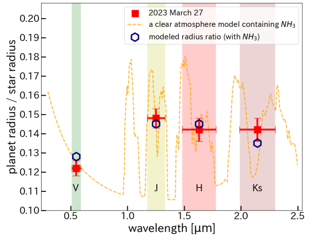
Fig. 3. Observed planet-to-star radius ratios of Qatar-1 b on March 27 compared to the clear atmospheric model spectrum. The red squares indicate the radius ratios observed on 2023 March 27. The orange dashed line represents a clear atmospheric model spectrum with H_2 99%, NH_3 1%, a mean molecular weight of 2.15 g/mol, planetary diameter of 114,100 km (0.7 times the original), an expansion factor b_s of 10, and pressure of 5.0 \times 10^{-1} bar. The dark blue hexagons show the radius ratios of the atmospheric model corrected for the filter transmittance in each band.
